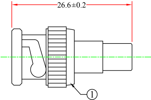
BNC Male to RCA Female Adapter
