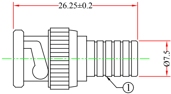
BNC Male
